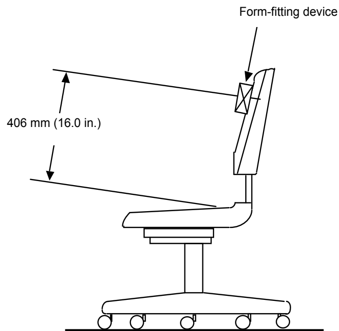
Figure 14b - Positioning of Form-Fitting Device for Backrests Higher than 452 mm (17.8 in.) Backrest Durability Test Cyclic - Type I
