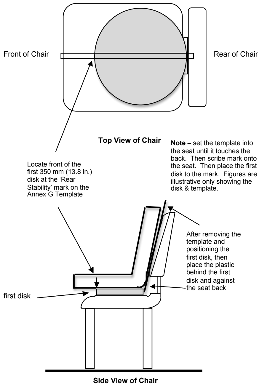
Figure 11a – Rear Stability First Disk Placement
